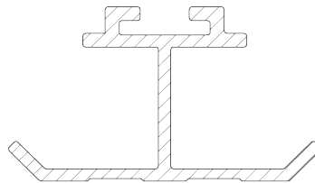
INTEGRATED STIFFENER
