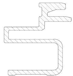
FRAME EXTRUSION
